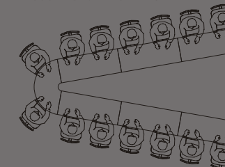
grupthink 15 seater table 4670 x 1915 x 740 mm ht.
